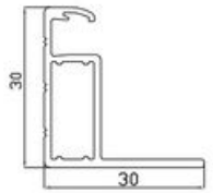
Section diagram of long frame profile
